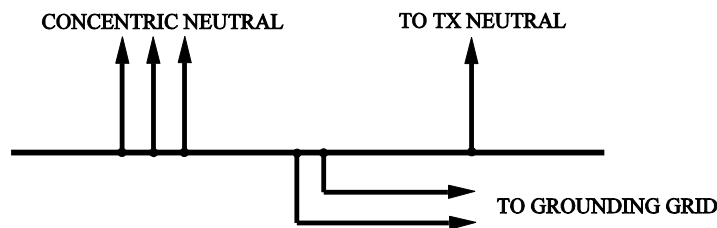
GROUNDING SCHEMATIC
